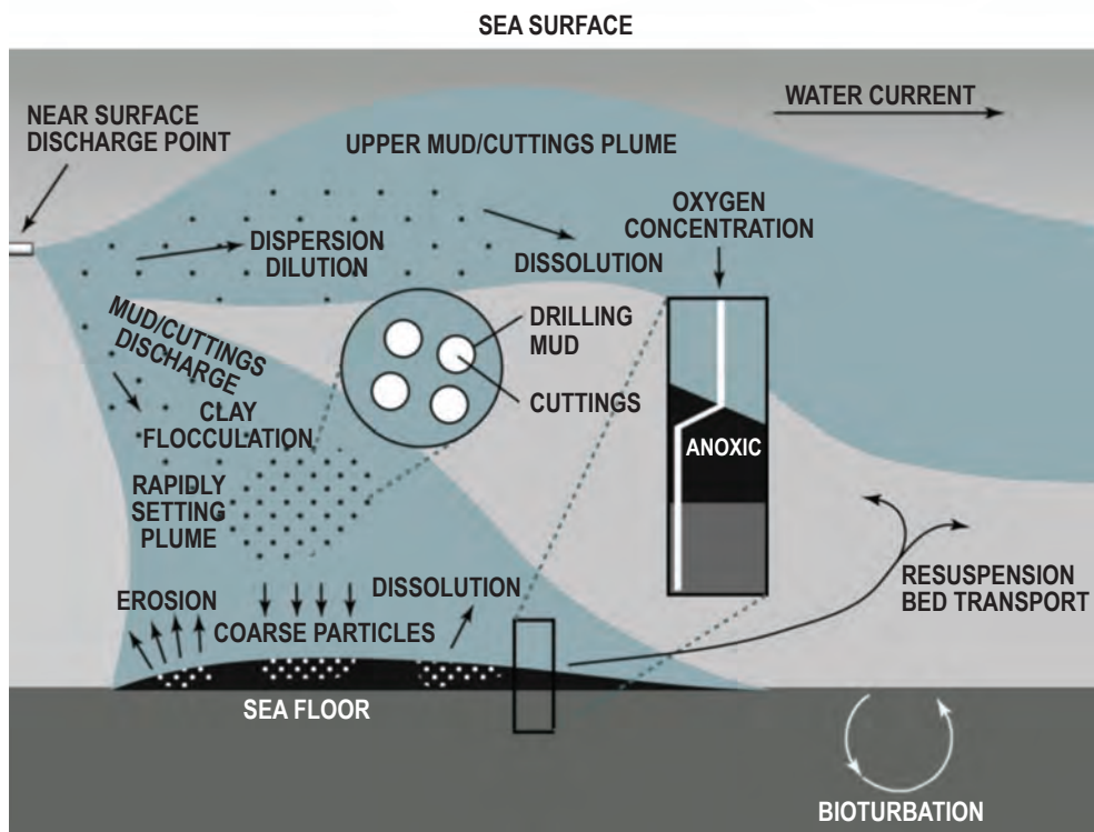
Figure 9-16. Dispersion and Fates of Water-Based Drilling Fluids and Drill Cuttings following Discharge to the Ocean
