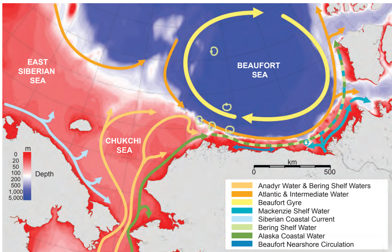
Figure 9-3. Summary of the Circulation and Water Masses in the Chukchi and Beaufort Seas
