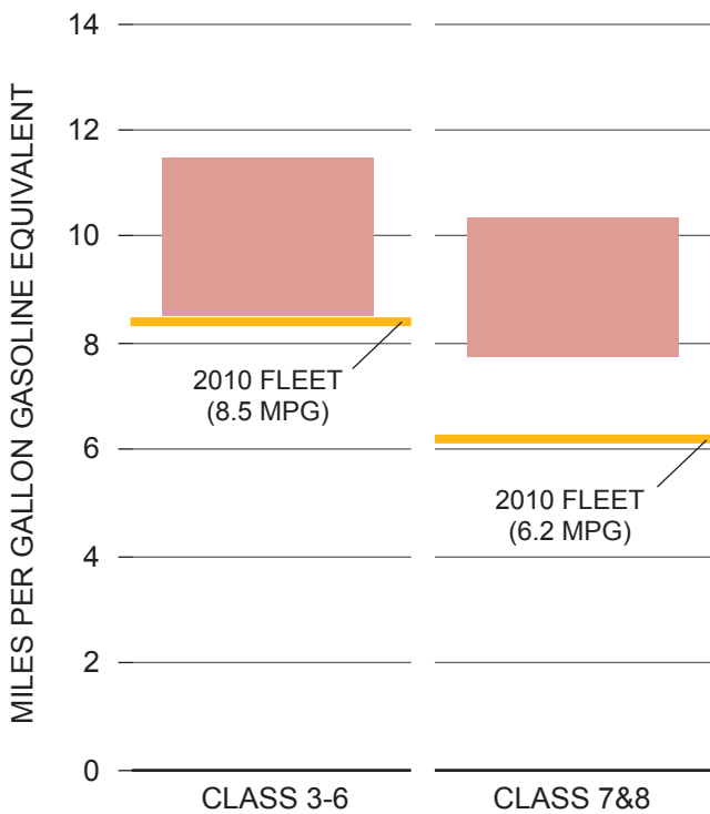
Figure ES-7. Range of Medium- and Heavy-Duty Vehicle On-Road Fleet Fuel Economy in 2050 (All Oil Prices)
