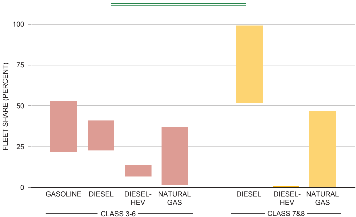
Figure ES-8. Range of Medium- and Heavy-Duty Vehicle Fleet Shares in 2050 (All Oil Prices)
