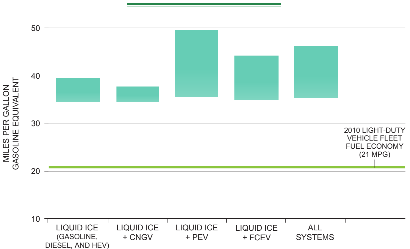
Figure ES-5. Range of Light-Duty Vehicle On-Road Fleet Fuel Economy in 2050 (3-Year, All Oil Prices)
