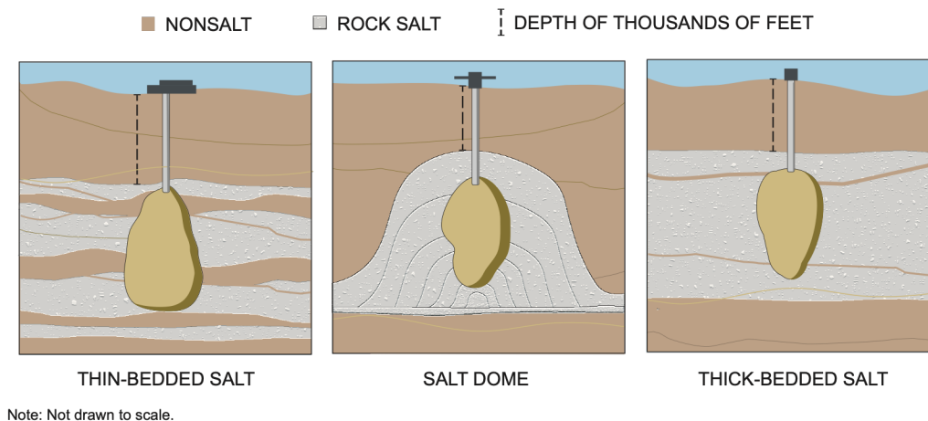
Figure 1-9. Bedded Salt Deposit and Bedded Salt Cavern
